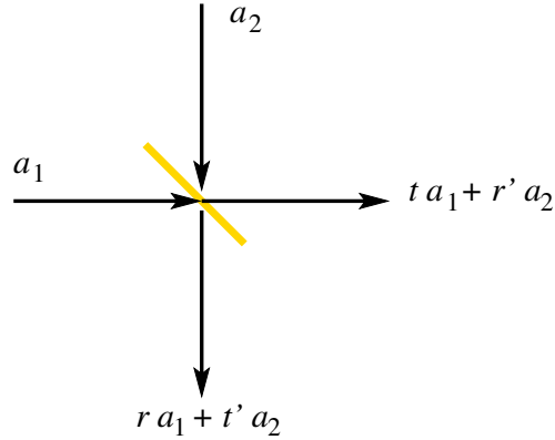
Figure 2.3: Mixing of two modes by a beam splitter.
