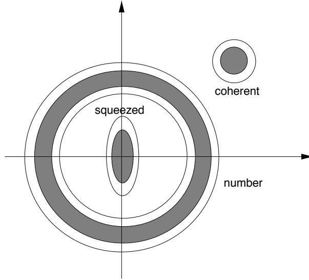
Figure 2.2: Quantum states of the radiation field, schematically represented in the phase space plane.
